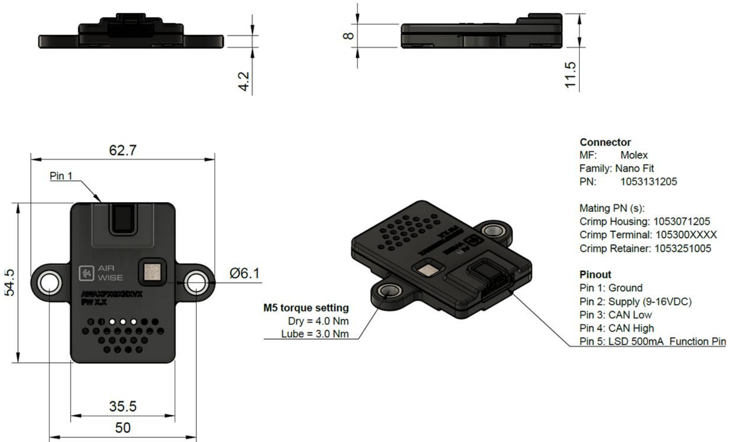
FIGURE 4 SENSOR DIMENSIONS
