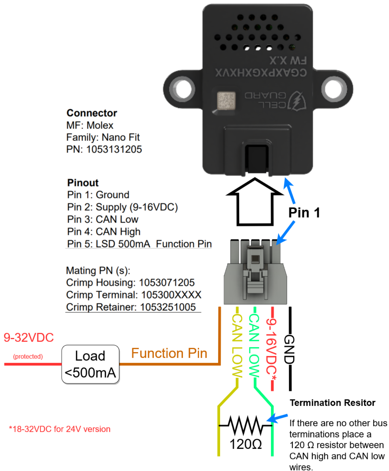
FIGURE 3 WIRING EXAMPLE
