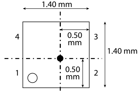
9.1 LGA Package
