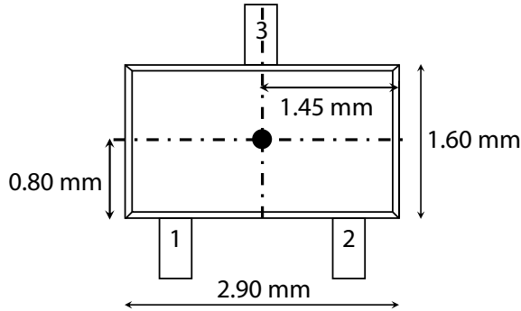
9.2 SOT Package
