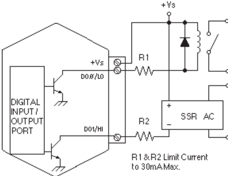
Figure 6.1 Digital Outputs Used With Relays
