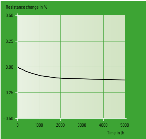
Long-term stability: MANGANIN® Typical long-term stability at +140 °C
