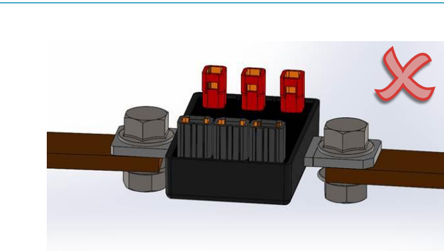
Figure 16 Incorrect mounting 15mm overlap
