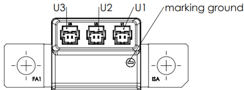
Figure 4: voltage measurement
