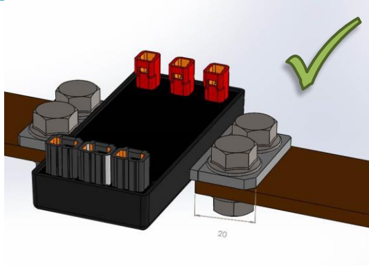
Figure 13 correct mounting 20mm overlap
