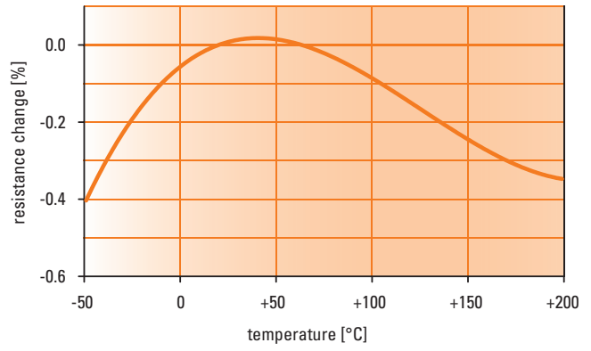
Graph 2: Electrical resistance vs. temperature (range -50 °C bis +200 °C)
